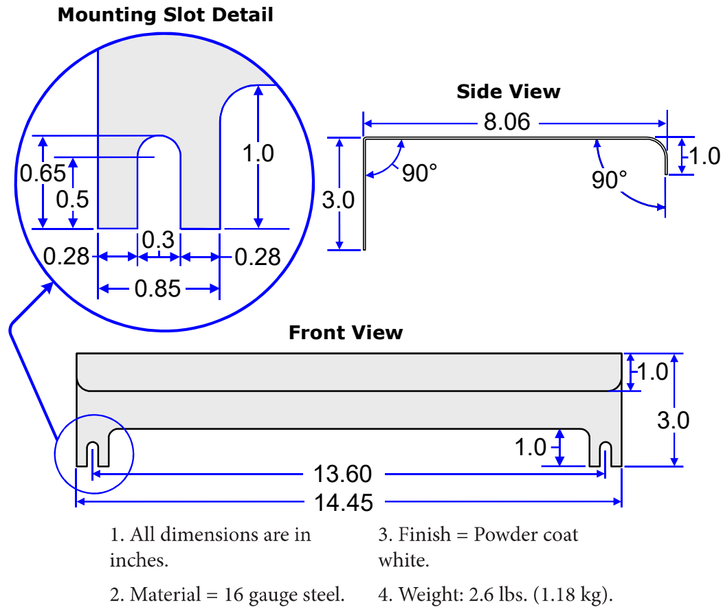
Figure 2, MP-HOOD Dimensions/Specs
